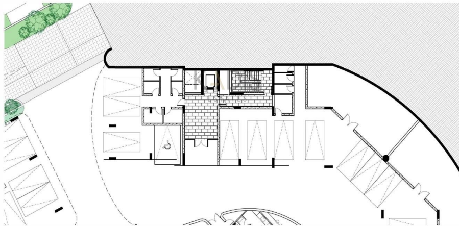
BUILDING D LOWER GROUND FLOOR
