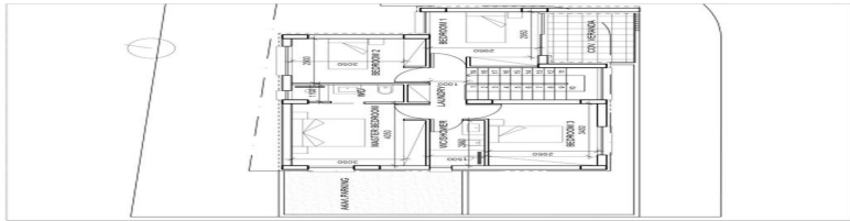
floor plan
