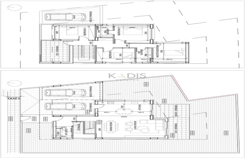
HOUSE C3 ground floor plan 1:100 floor plan
