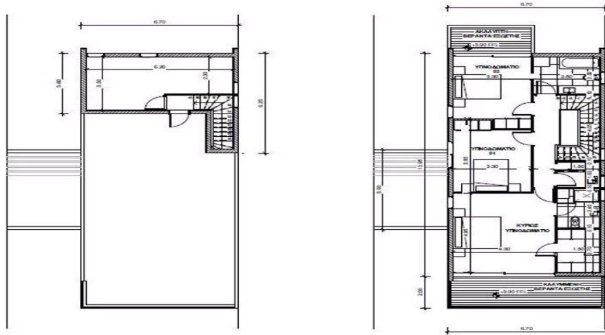
SECOND FLOOR A1 1:100
