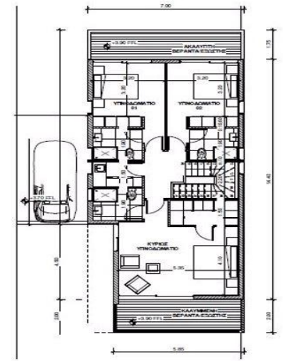
FIRST FLOOR B1/B2 1:100
