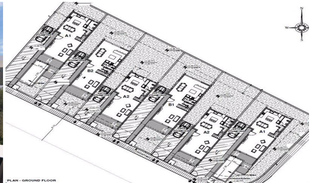
PLAN - GROUND FLOOR
