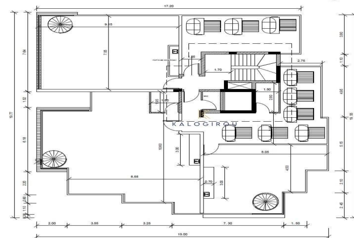
1 ROOF GARDEN 1:100
