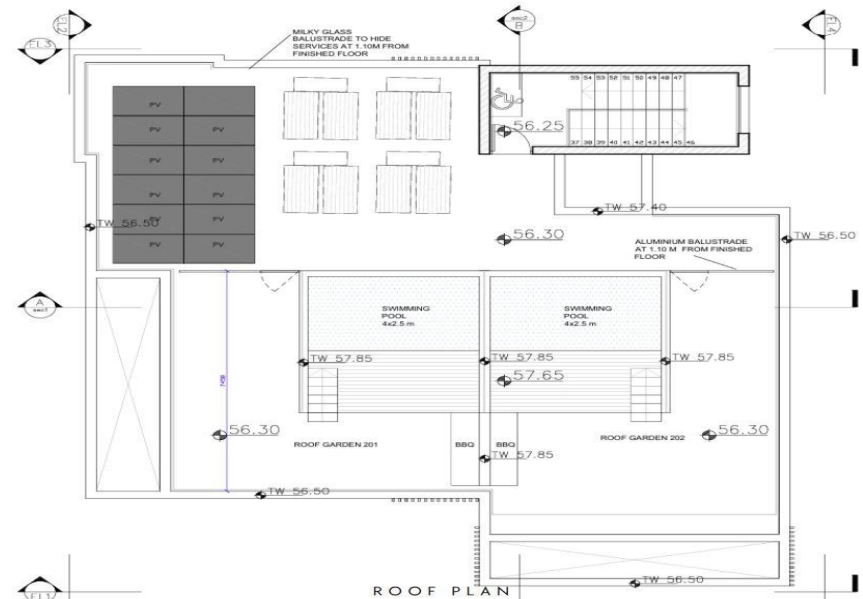
ROOF PLAN
