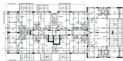
1st Floor (block A)
