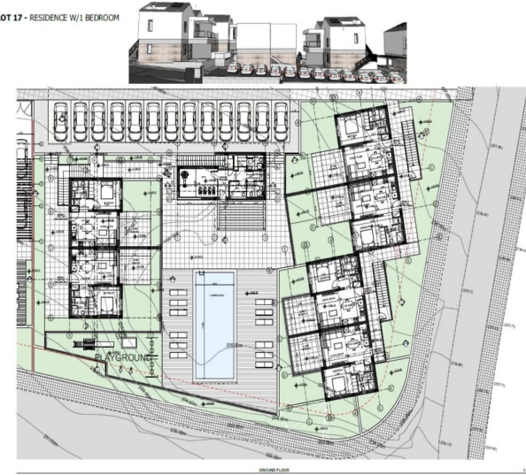
PLOT 17 - RESIDENCE W/1 BEDROOM
