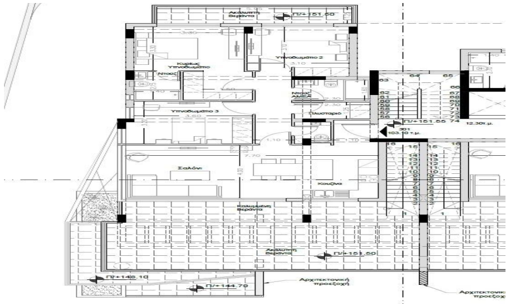
Ground Level
