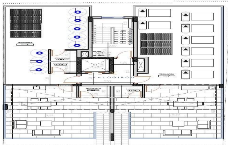
ROOF GARDEN PLAN
