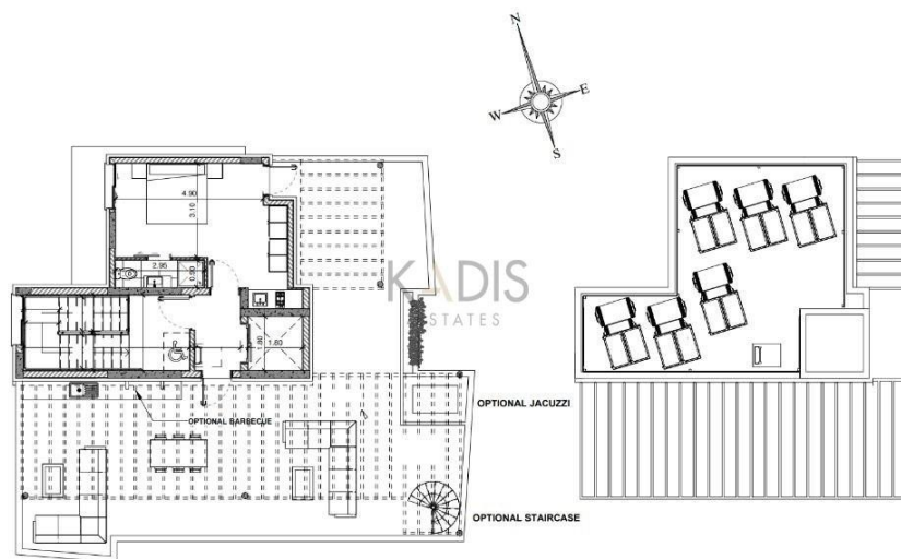
ROOF PLAN
