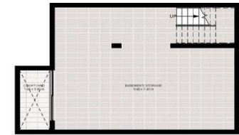
3 Basement Basement Area: 30 m² (3m2) Courtyard Area: 7 m²
