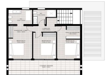
2 1st Floor 1st Floor Area: 80 m² (8m2) Covered Veranda Area: 15 m²
