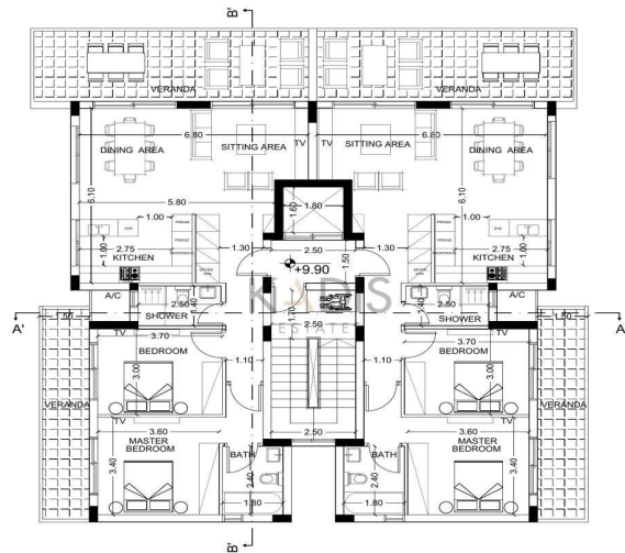
THIRD FLOOR
