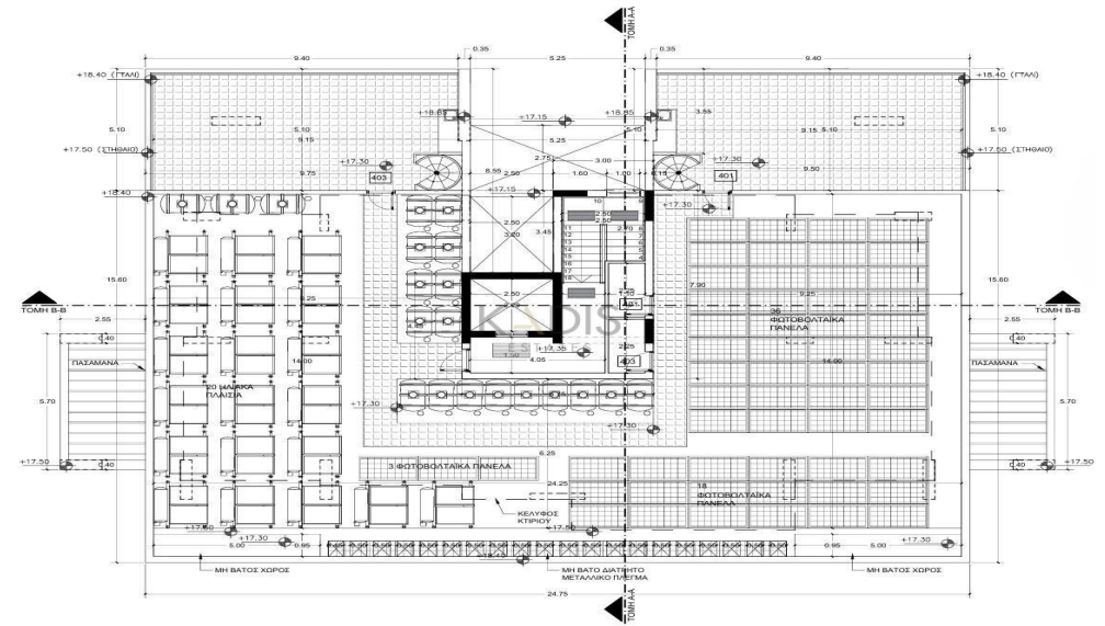
ROOF PLAN
