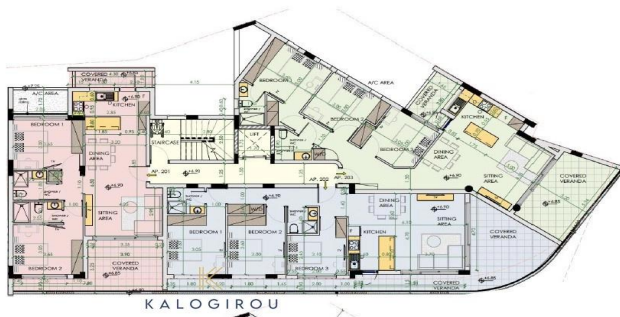
Floor Plan FLOORS 2
