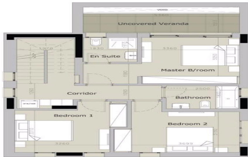
1st floor
