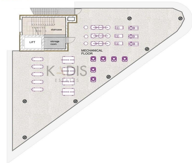
MECHANICAL
