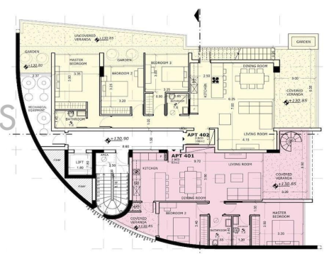
FLOOR PLANS FOURTH FLOOR
