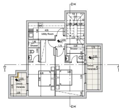
BASEMENT FLOOR
