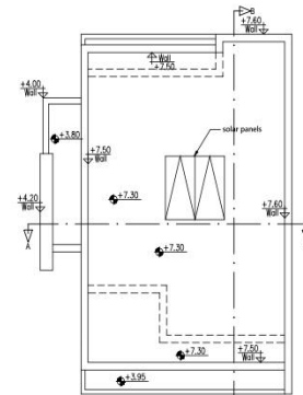
ROOF PLAN
