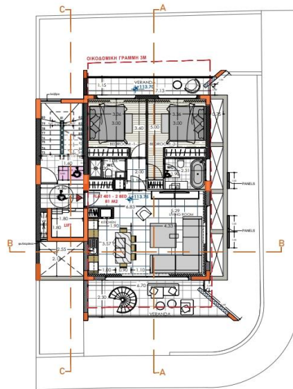
FORTH FLOOR PLAN
