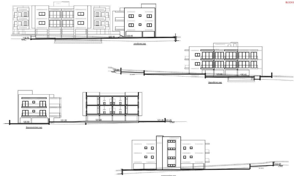
BLOCK B
