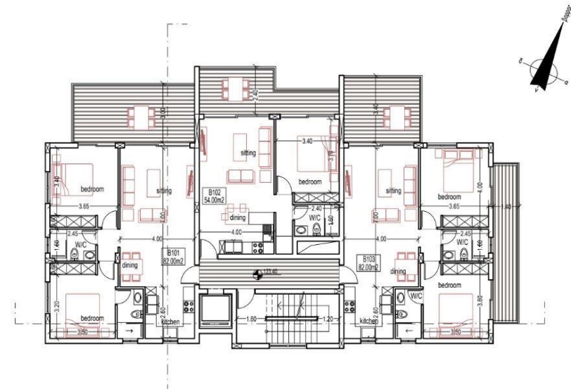
BLOCK B
