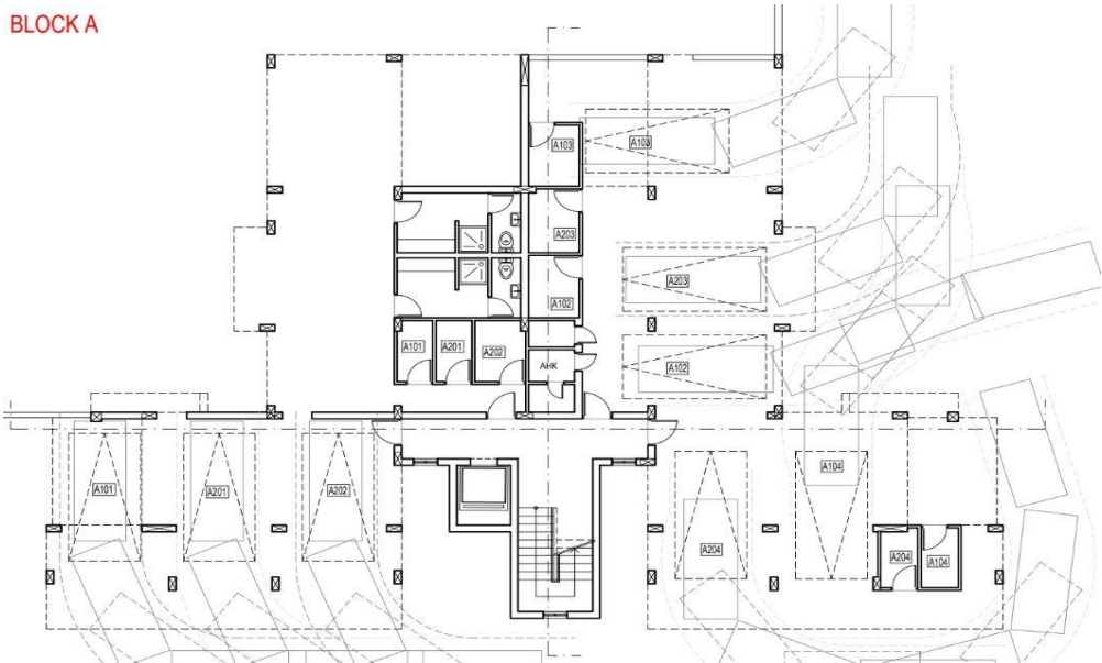
BLOCK A
