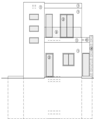
BACK ELEVATION
