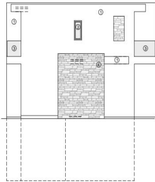
LEFT ELEVATION
