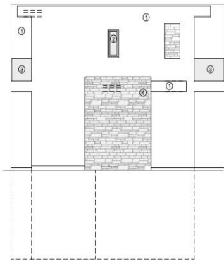
LEFT ELEVATION
