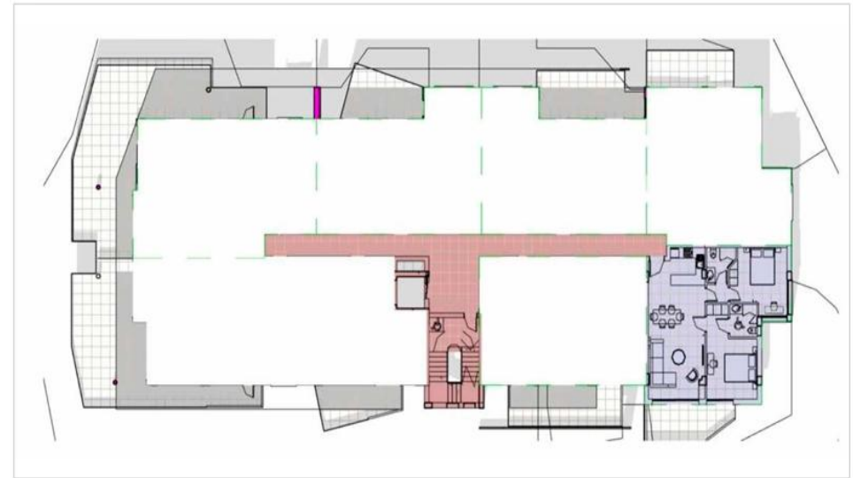
PRELIMINARY SECOND FLOOR LAYOUT PLAN
