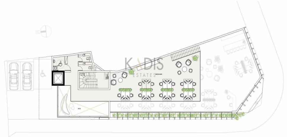
MEZZANINE FLOOR
