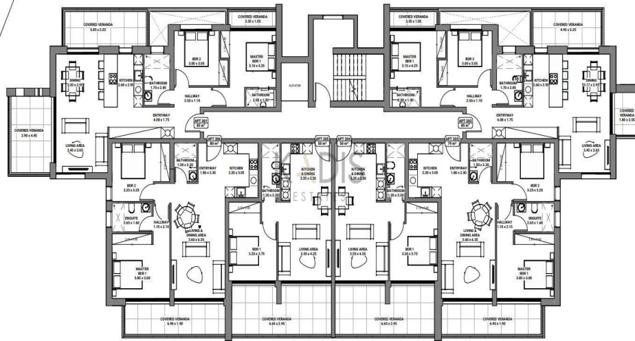
1 Brochure-Second Floor Plan 1:100
