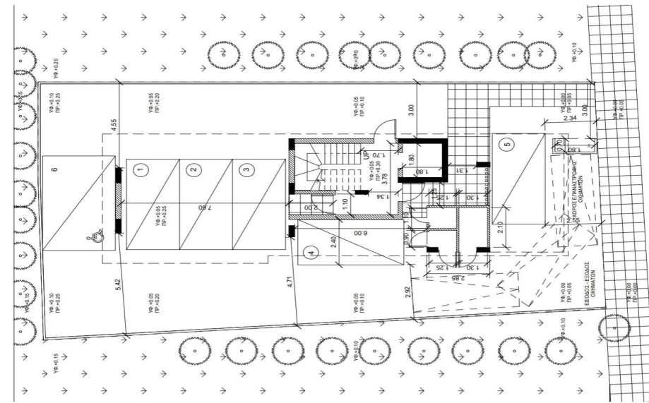
PLANS GROUND FLOOR
