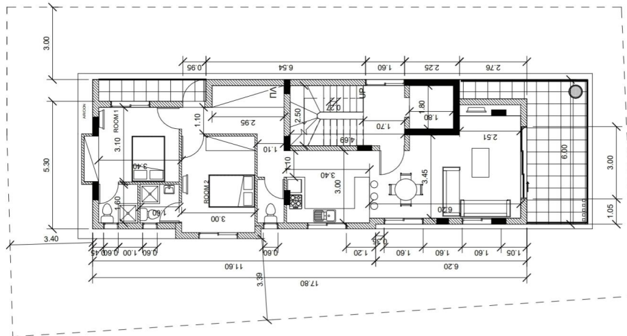
PLANS SECOND FLOOR
