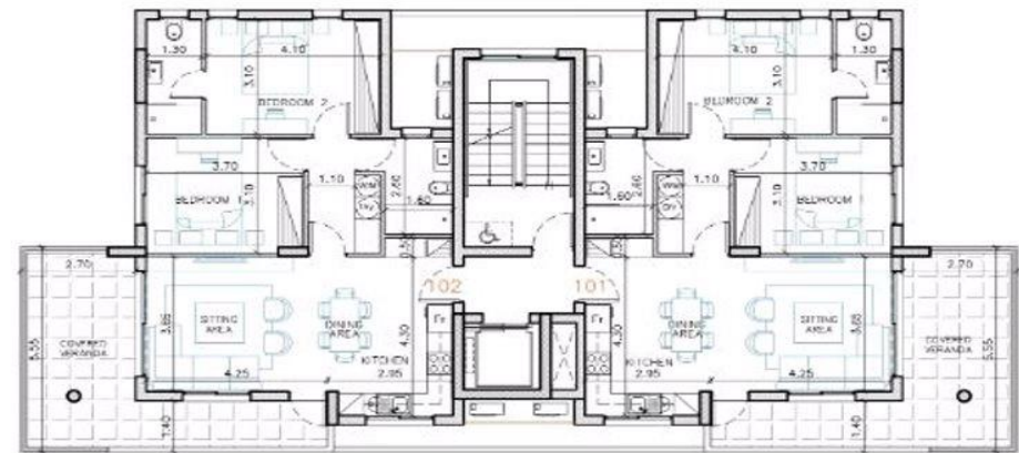
1st FLOOR PLAN 1:100
