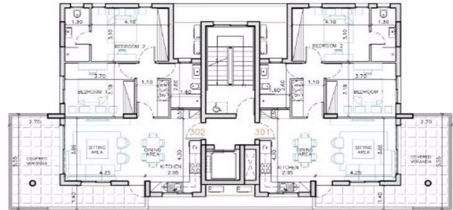
3rd FLOOR PLAN 1:100
