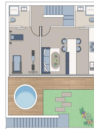
Lower Floor Plan
