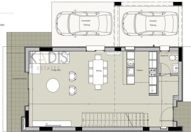
:ground level
