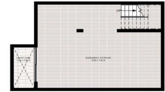
3 Basement Basement Area: 90 m 2 (8m 2 Staircase) Courtyard Area: 7 m 2
