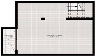
3 Basement Basement Area: 90 m² (9m2) Courtyard Area: 7 m²
