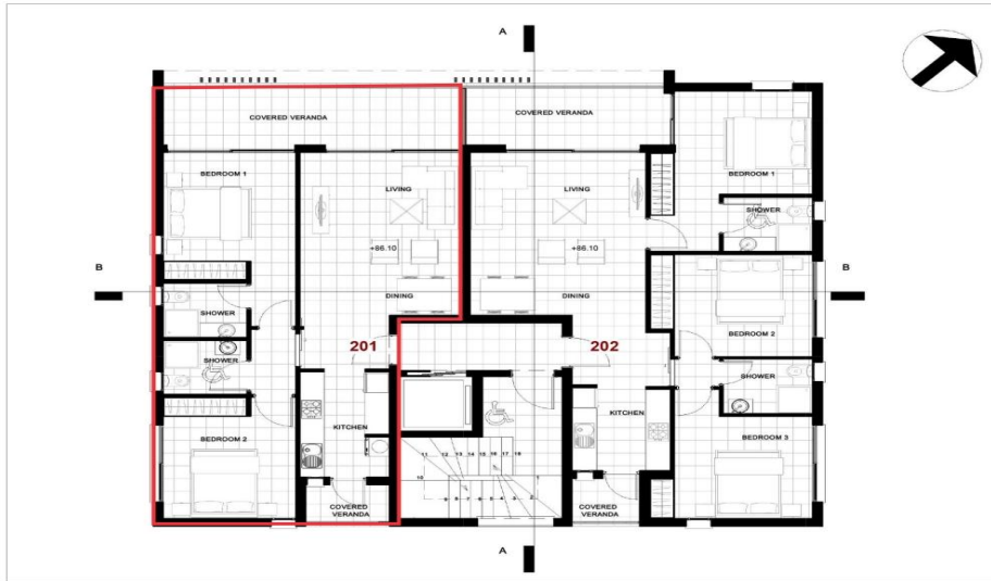
PRELIMINARY SECOND FLOOR PLAN
