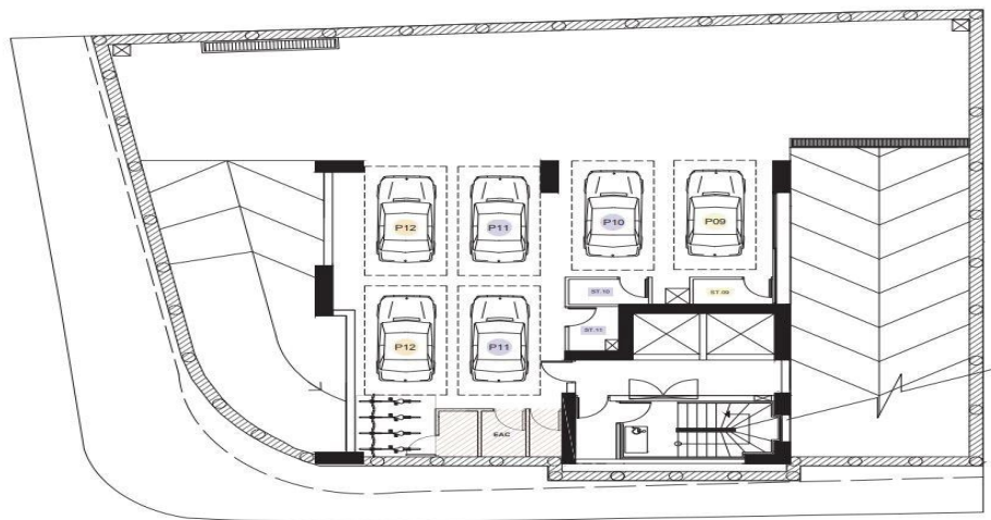
-1 BASEMENT PLAN SCALE 1:100
