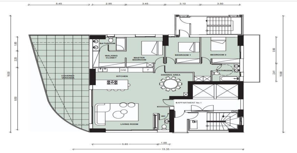
1st FLOOR PLAN SCALE 1:100
