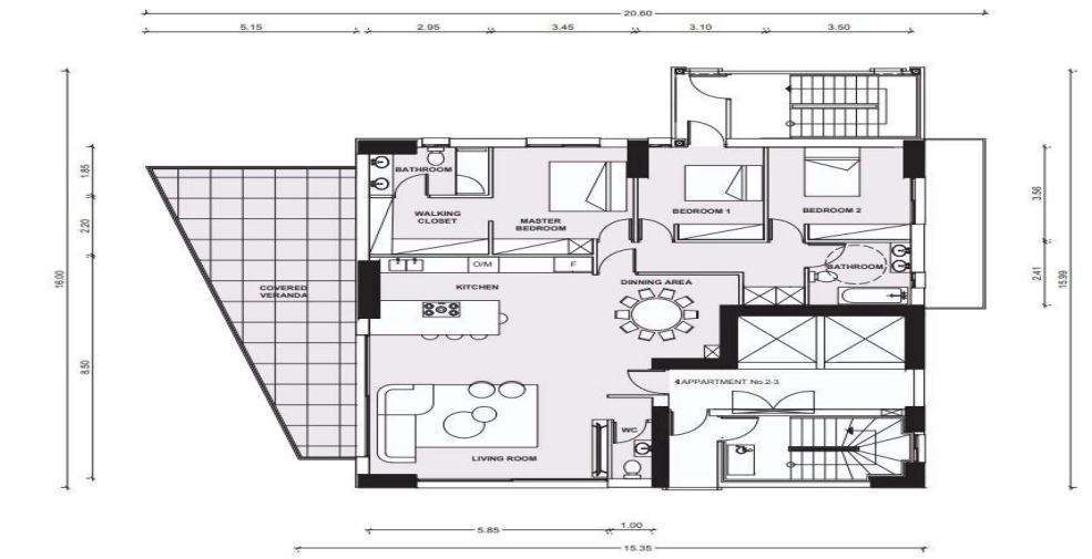
2nd-3rd FLOOR PLAN SCALE 1:100
