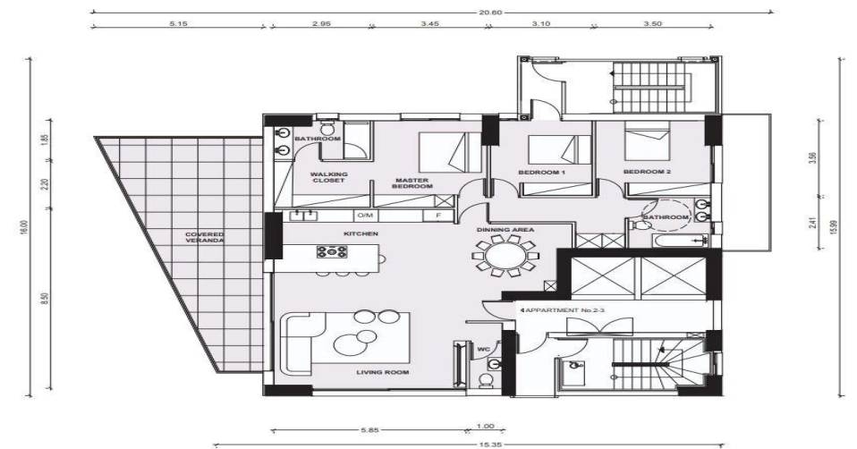
2nd-3rd FLOOR PLAN SCALE 1:100
