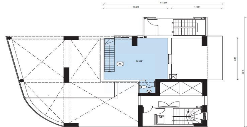
MIDDLE FLOOR PLAN SCALE 1:100
