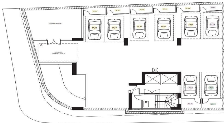
-2 BASEMENT PLAN SCALE 1:100
