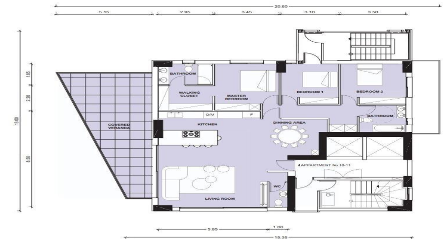
10th-11th FLOOR PLAN SCALE 1:100
