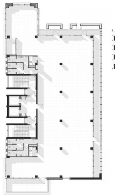
2ND - 5TH FLOOR
