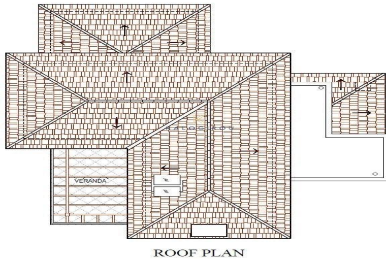
ROOF PLAN
