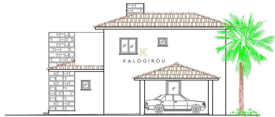
SIDE ELEVATION
