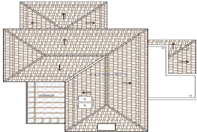
ROOF PLAN
