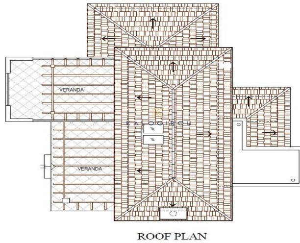
ROOF PLAN
