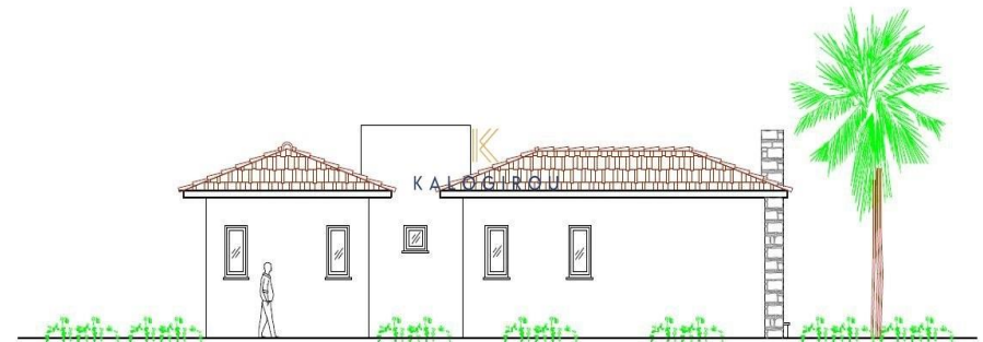
BACK ELEVATION
