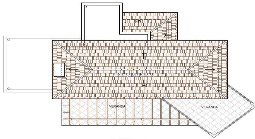
ROOF PLAN
