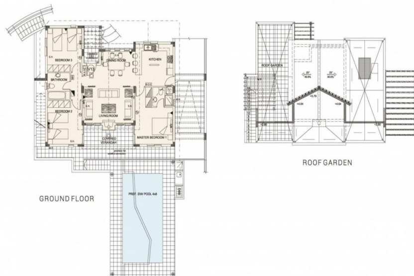
3 BEDROOM VILLA
