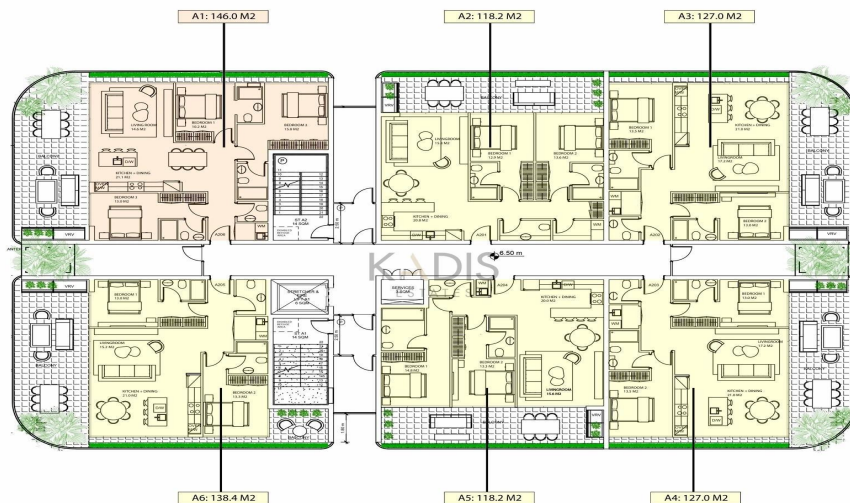
1 LEVELS 02-08 1:100
