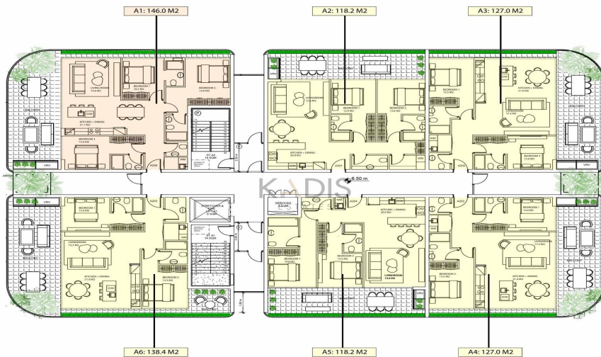
1 LEVELS 02-08 1:100
