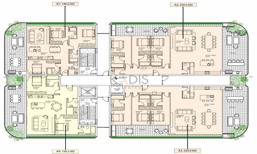
1 LEVEL 09 1:100
