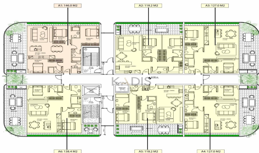
LEVELS 02-08 1:100
