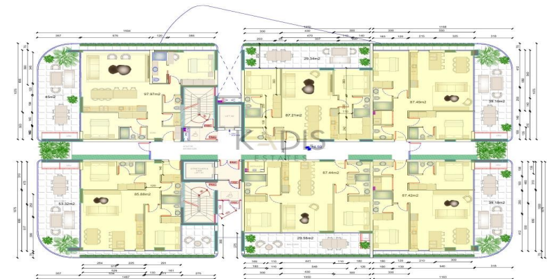
2nd-8th FLOOR
