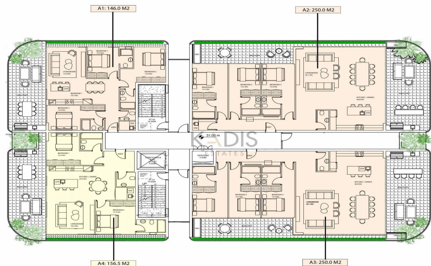
LEVEL 09 1:100
