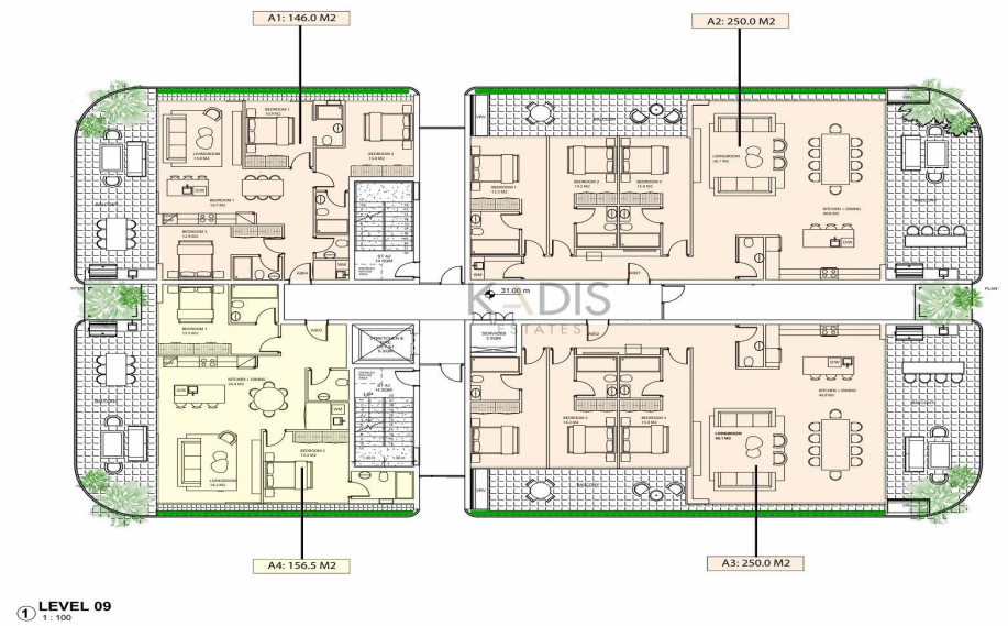
LEVEL 09 1:100
