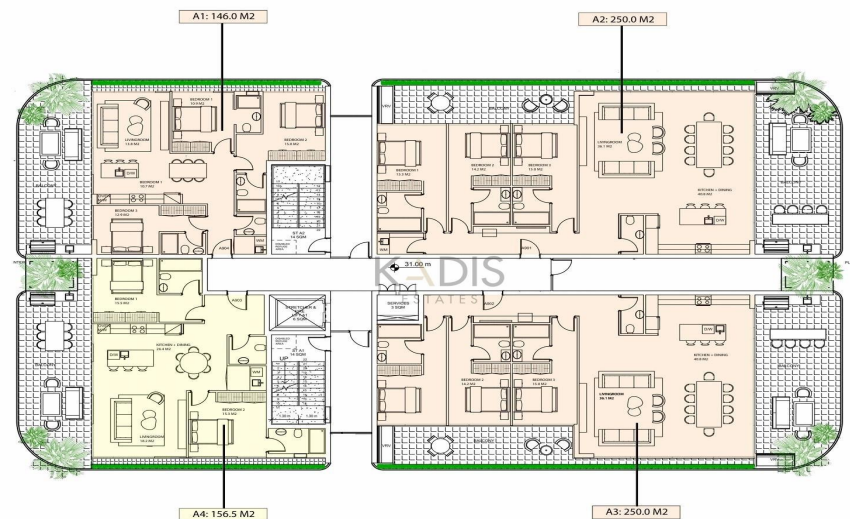
① LEVEL 09 1:100
