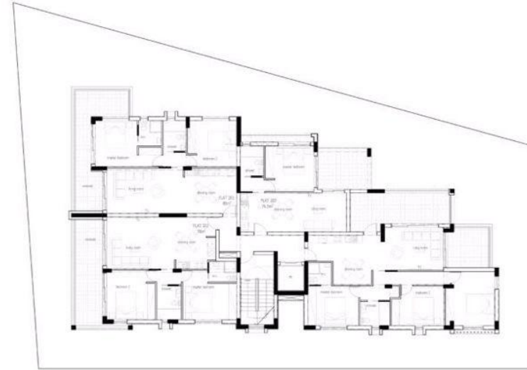
Second Floor Plan for Block
