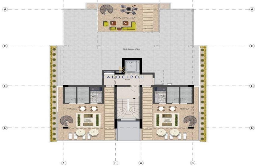
ROOF FLOOR PLAN
