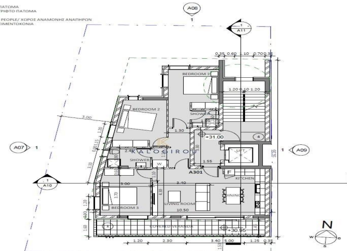
1 3. Third Floor 1 : 100
