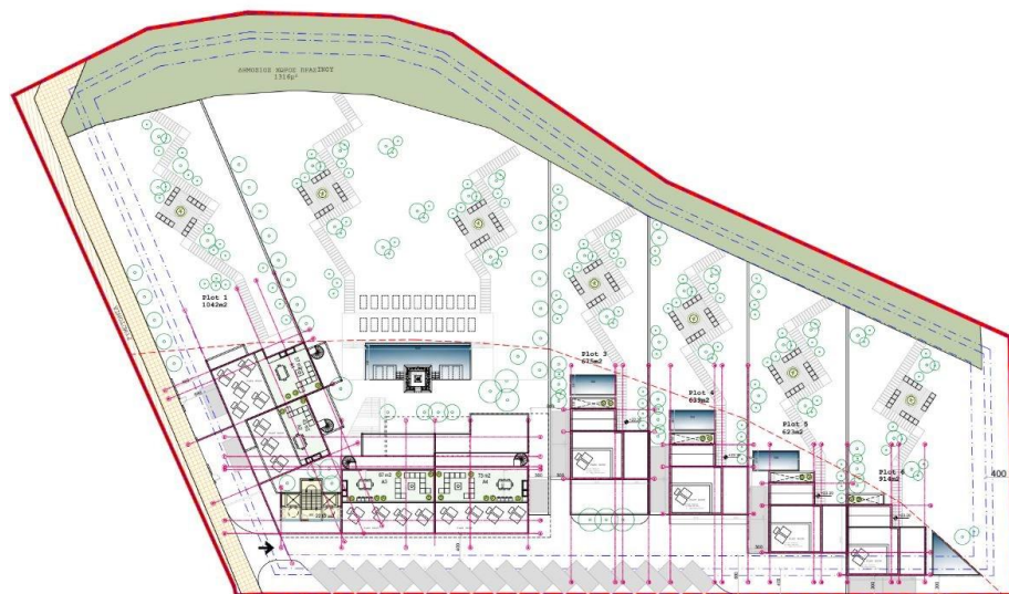
ROOF PLAN
