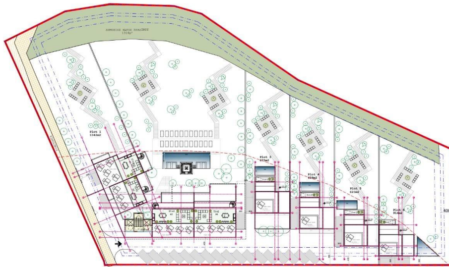
ROOF PLAN
