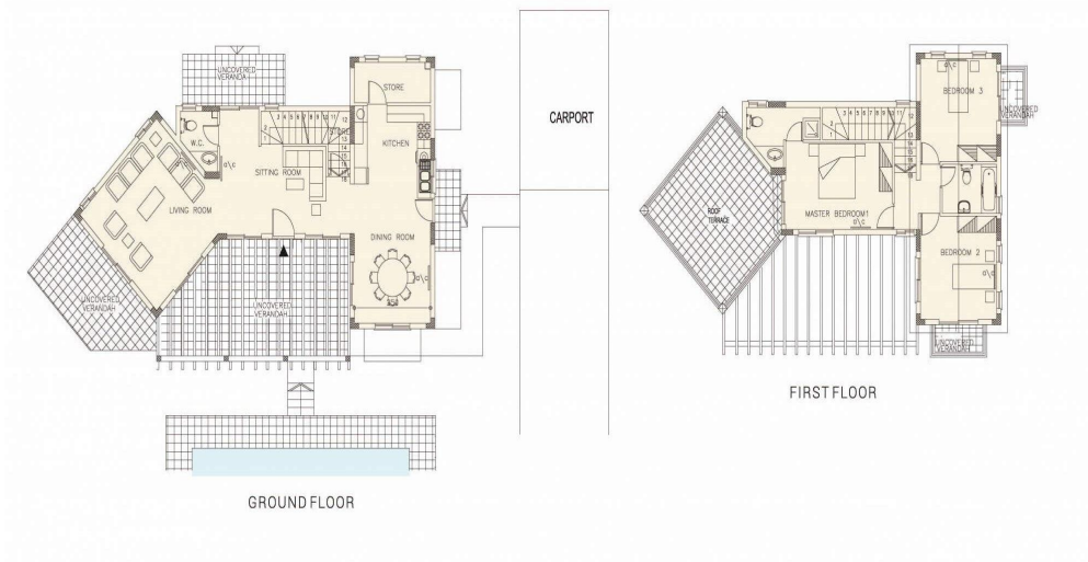
3 BEDROOM VILLA
