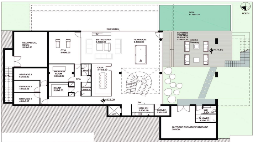
BASEMENT PLAN
